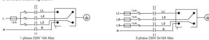
3 circuit track system
