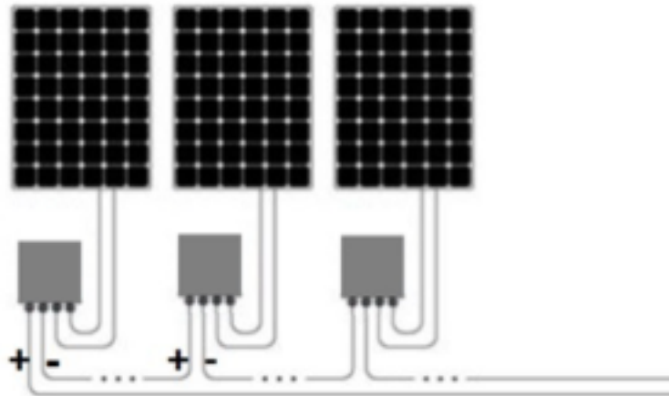
Figuur 5 Power Optimizer in series verbonden
